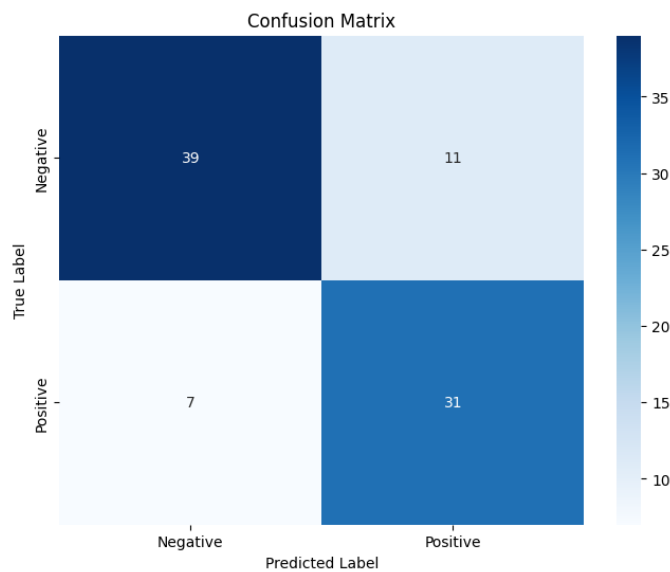
Figure 4: Confusion matrix
