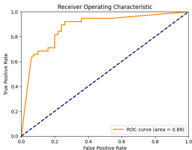
Figure 5: ROC-AUC
